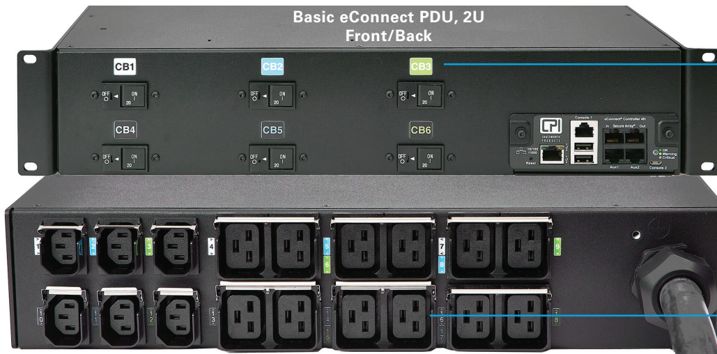
Hydraulic-Magnetic Breakers
